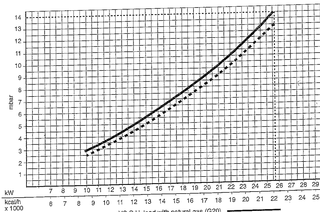
Fig 5 - Burner pressure VS C.H. load with natural gas (G20)
