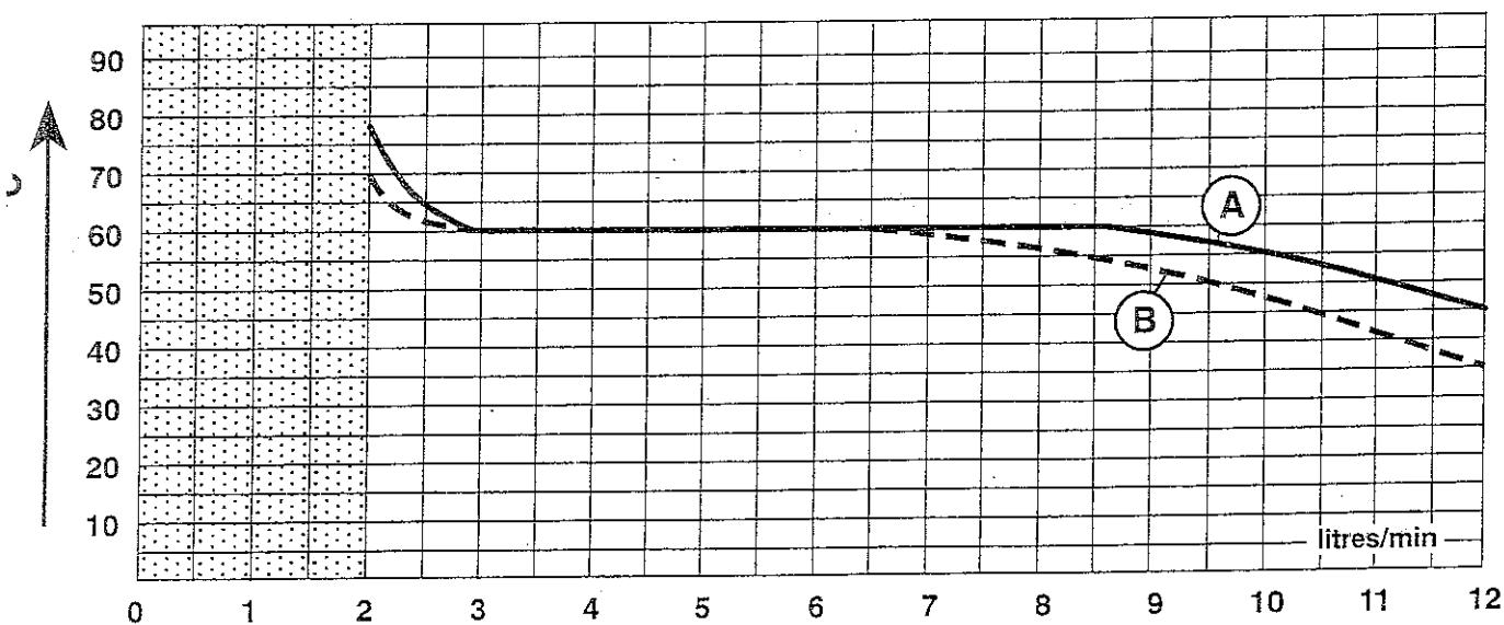
Fig 2 - D.H.W. temperature VS. flow A = Cold Water 15°C B = Cold Water 5°C
