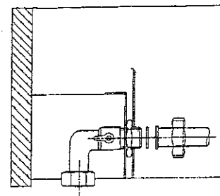
4 = Domestic Cold Water inlet 1/2" 6 = Central Heating flow outlet 22 mm 7 = Central Heating return inlet 22 mm
