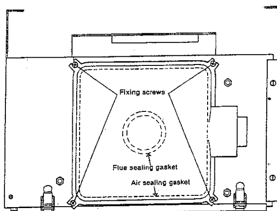
TOP VIEW BOILER SIDE OUTLET
