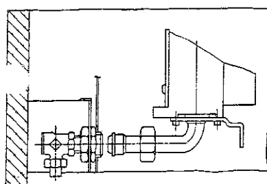
2 = Gas 3/4" B.S.P
