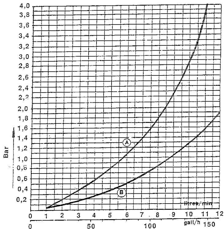
Fig 1 - D.H.W. Pressure Drop VS. flow A = Standard with cold water Flow Restrictor 10 l/min B = Cold Water Flow Restrictor Removed
