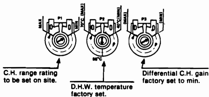
Fig. 3 - Potentiometers settings.
