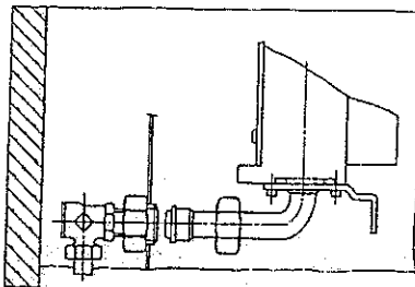
2 Gas 3/4" B S P.
