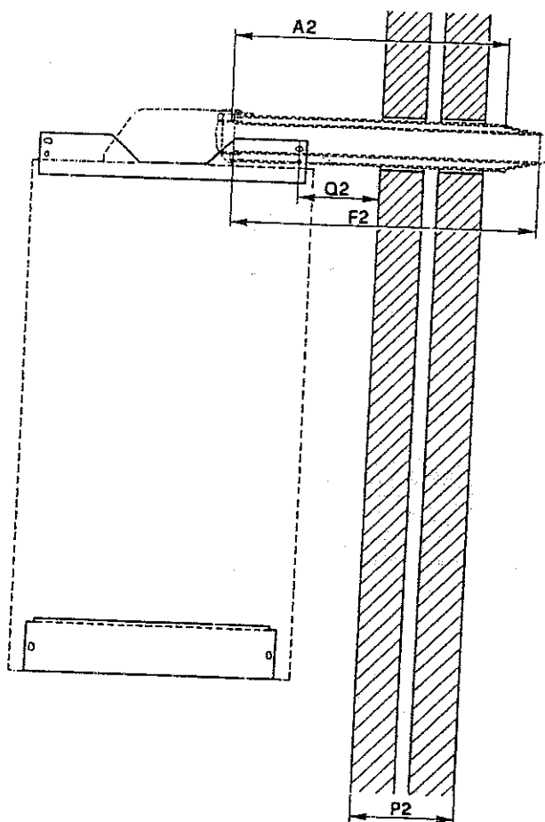
Side Flue Outlet
